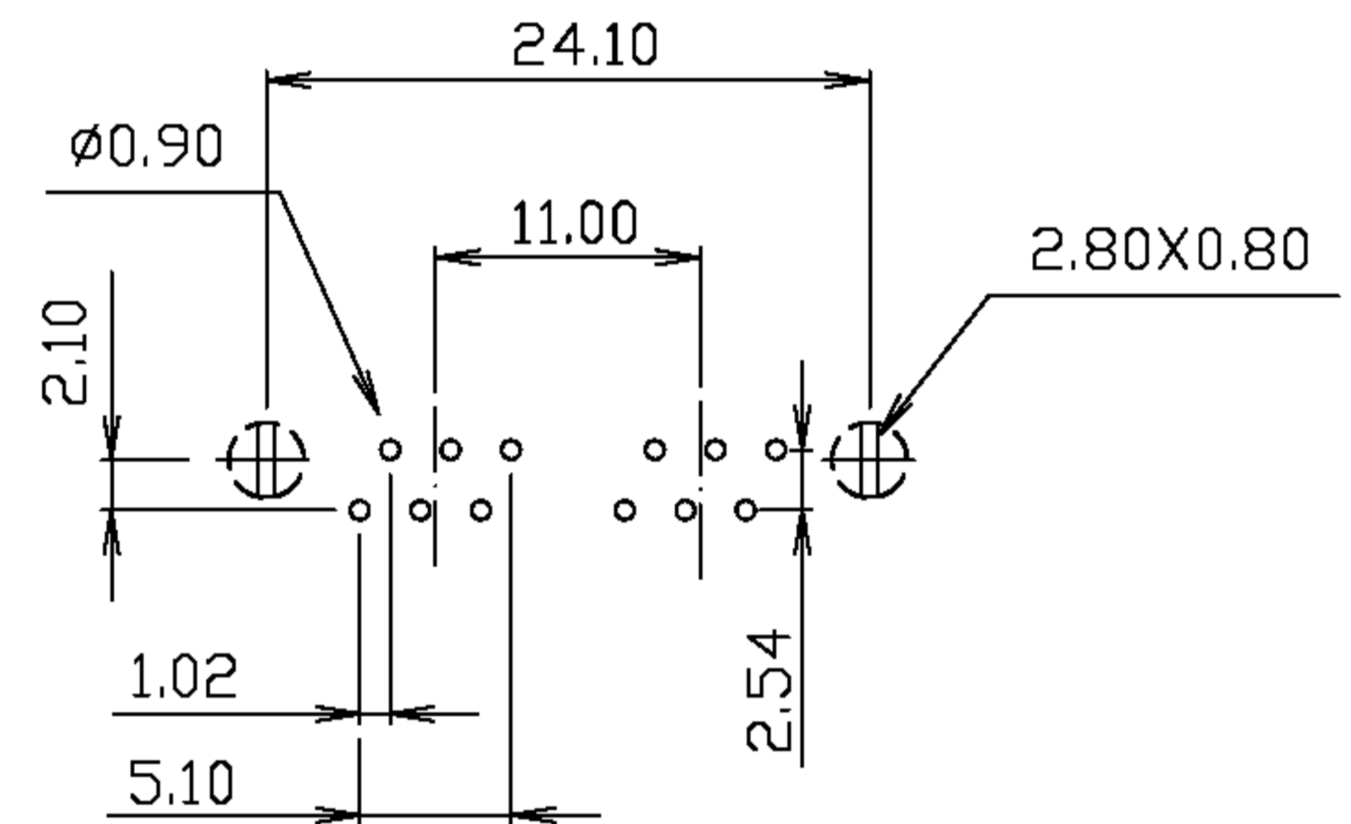
PC Board Layout
