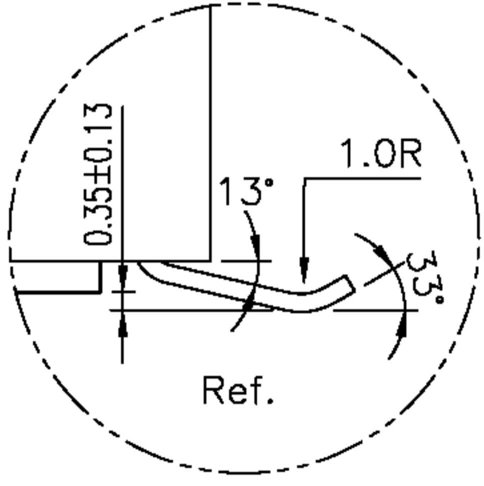
DETAIL X
