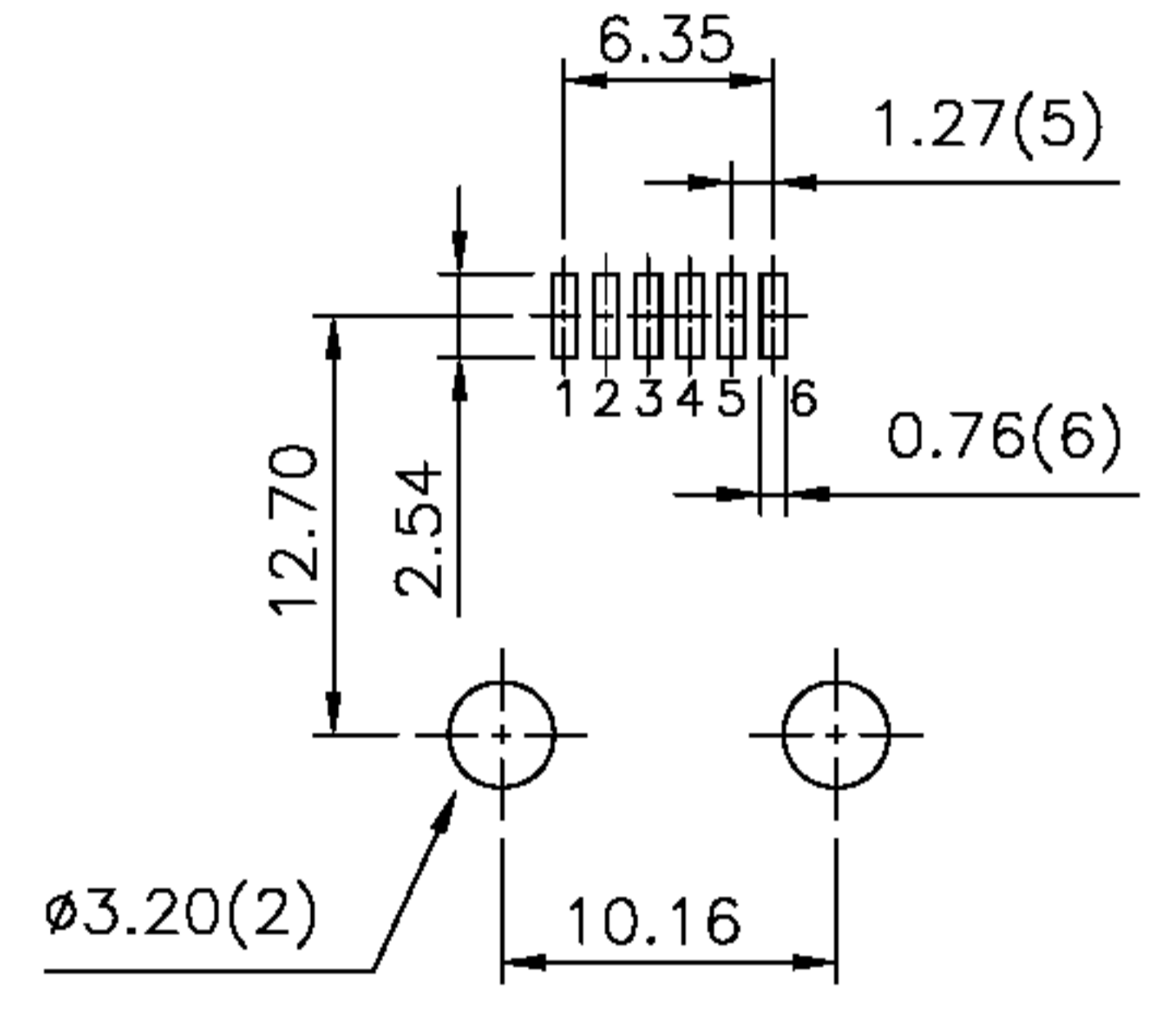
PCB LAYOUT Ref.
