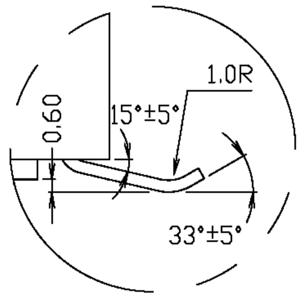
DETAIL X
