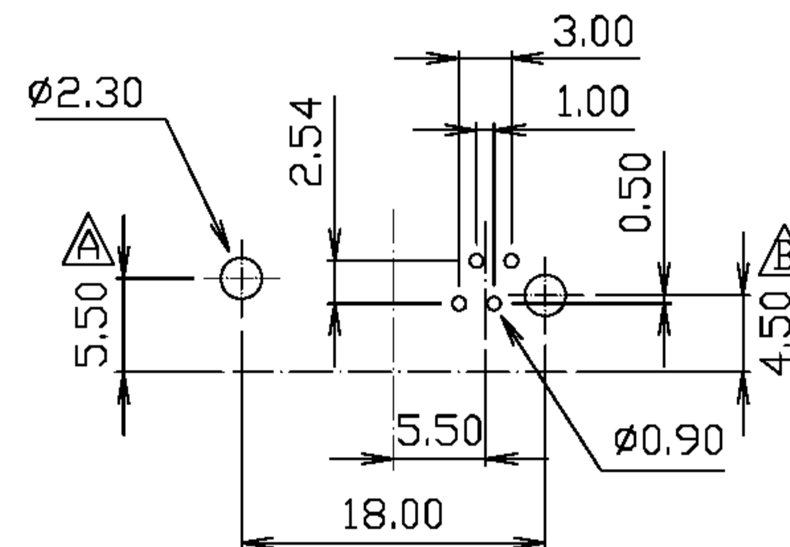
PC Board Layout
