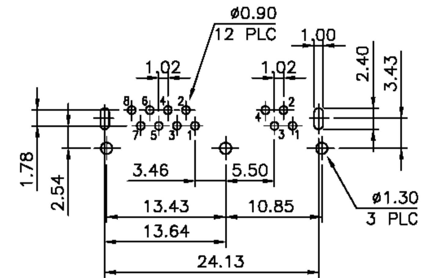
PCB LAYOUT Ref.
