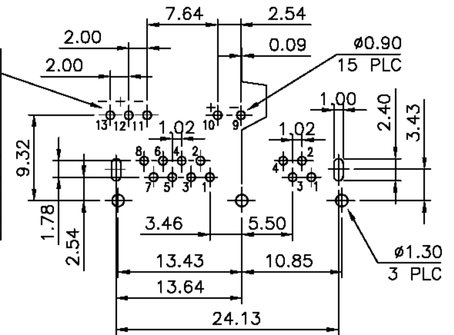
PCB LAYOUT Ref.
