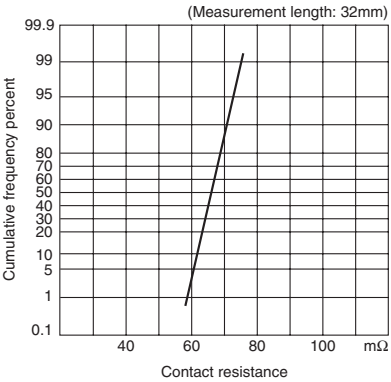
(2) Contact resistance
