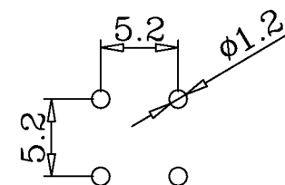
LAYOUT
