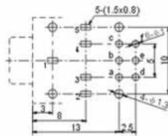
P.C.B Layout (copper-sided view)
