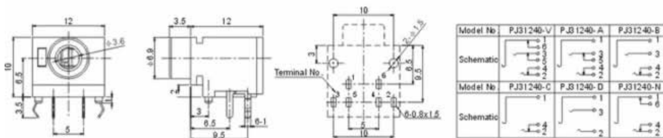
P.C.B Layout(copper-side view)
