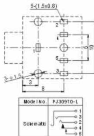
P.C.B Layout(copper-sided view)
