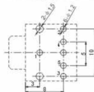
P.C.B Layout(copper-sided view)
