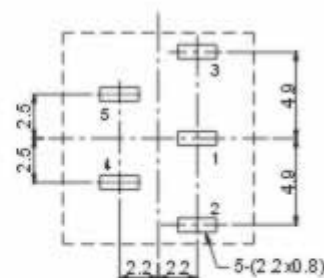
P.C.B. Layout (copper-side view)
