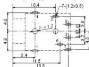
P.C.B Layout(copper-sided view)
