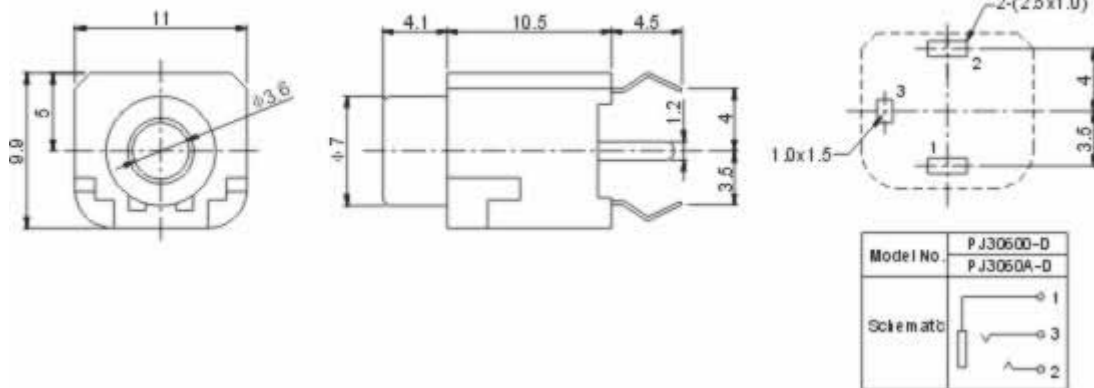
P.C.B Layout(copper-sided view)
