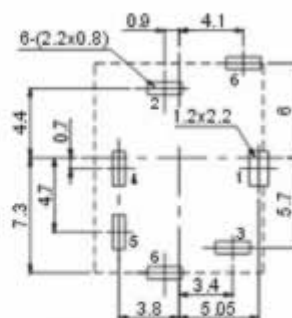
P.C.B Layout(copper-sided view)
