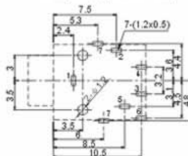
P.C.B Layout(copper-side view)
