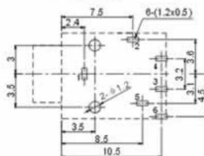
P.C.B Layout (copper-side view)
