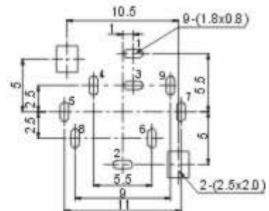
P.C.B Lay out (copper-side view)
