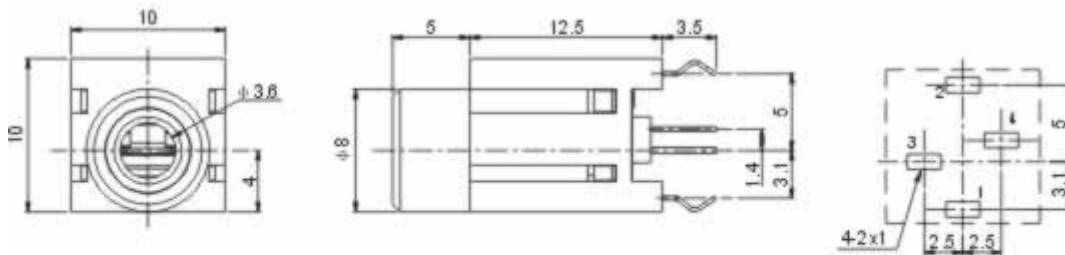
P.C.B Layout(copper-side view)
