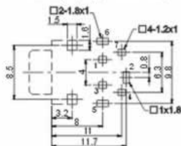
P.C.B Layout (copper-sided view)
