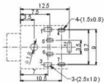
P.C.B Layout(copper-side view)
