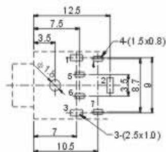
P.C.B Layout(copper-side view)
