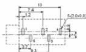
P.C.B Layout(copper-sided view)
