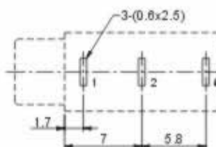
P.C.B Layout (copper-sided view)
