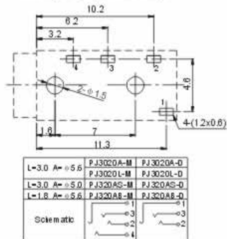
P.C.B Layout (Copper-side view)
