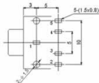
P.C.B Layout(copper-side view)
