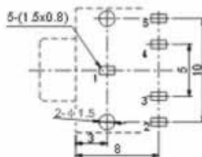
P.C.B Layout(copper-sided view)
