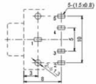
P.C.B Layout (copper-sided view)
