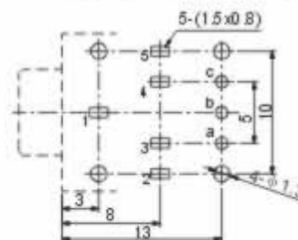
P.C.B Layout(copper-sided view)
