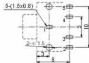
P.C.B Layout(copper-sided view)
