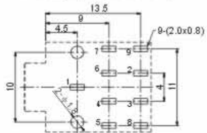
P.C.B Layout(copper-side view)
