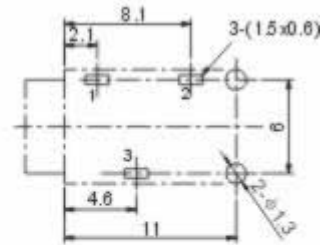
P.C.B Layout(copper-side view)
