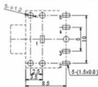
P.C.B Layout(copper-sided view)
