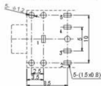
P.C.B Layout(copper-sided view)
