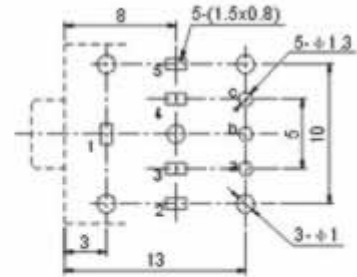
P.C.B Layout(copper-sided view)
