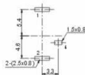
P.C.B Layout (copper-sided view)
