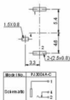
P.C.B Layout(copper-sided view)
