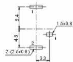
P.C.B Layout(copper-sided view)
