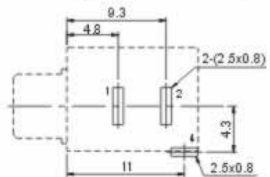
P.C.B Layout(copper-sided view)
