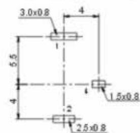
P.C.B Layout(copper-sided view)
