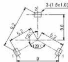
P.C.B Layout(copper-sided view)
