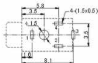
P.C.B Layout (copper-sided view)
