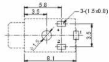
P.C.B Layout(copper-sided view)
