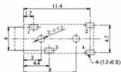
P.C.B Layout(copper-sided view)
