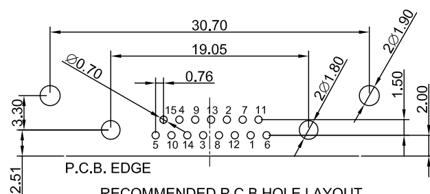
RECOMMENDED P.C.B HOLE LAYOUT COMPONENT SIDE VIEW(TOLERANCE ±0.05mm)
