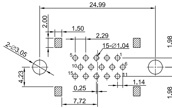
LAYOUT (COMPONENT SIDE VIEW) TOLERANCE : \pm 0.10
