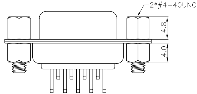
RIVETED #4-40 NUTS WITH JACK SCREWS
