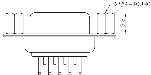
RIVETED FRONT #4-40 NUTS
