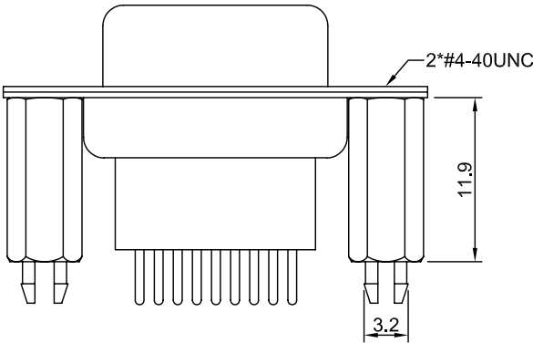
RIVETED #4-40 NUTS 11.9mm STAND OFF BOARD LOCK
