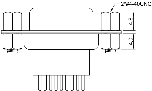
RIVETED #4-40 NUTS WITH JACK SCREWS
