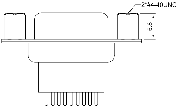
RIVETED FRONT #4-40 NUTS
