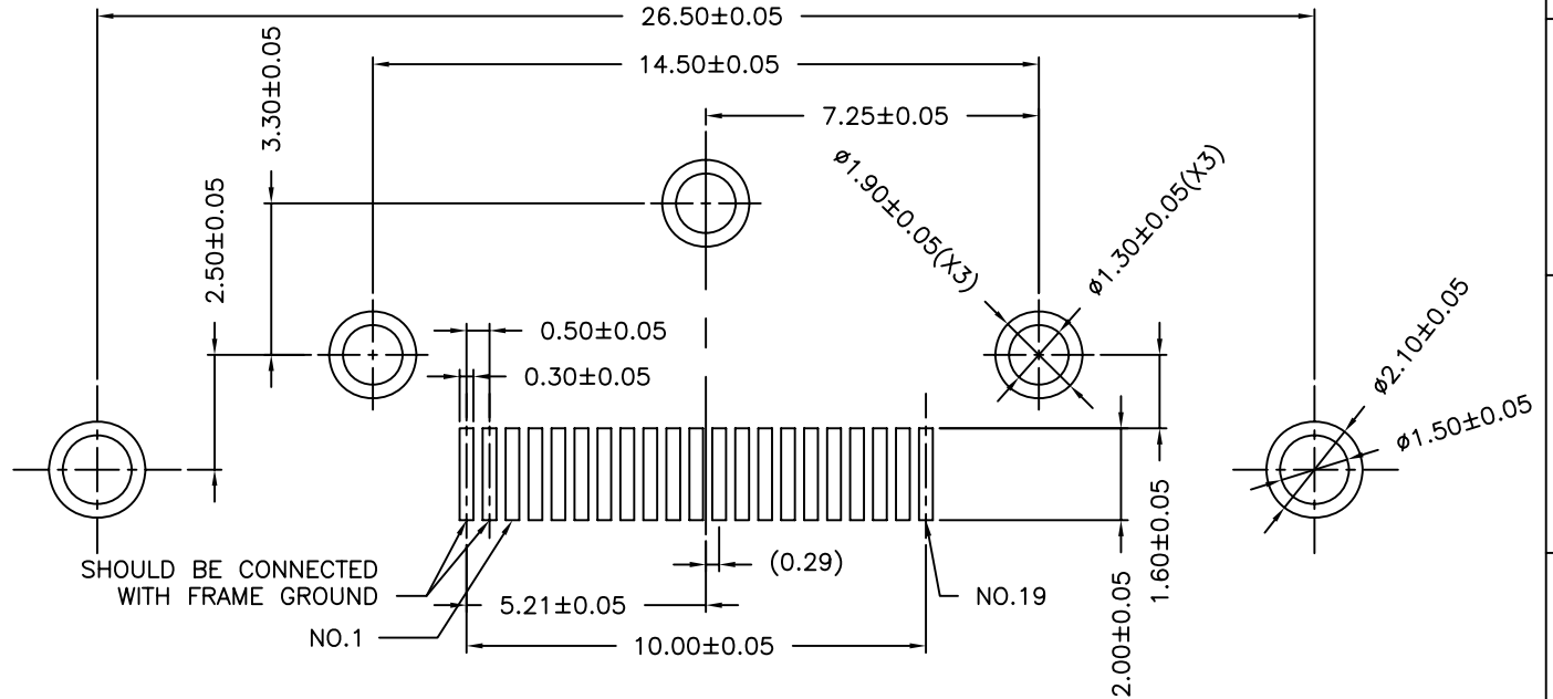
RECOMMENED P.C.B. LAYOUT(T=1.6mm)
